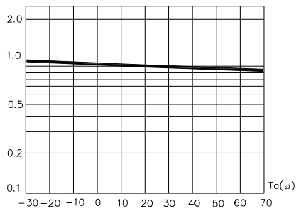
Fig.5 Relative Luminous Intensity vs. Ambient Temperature
